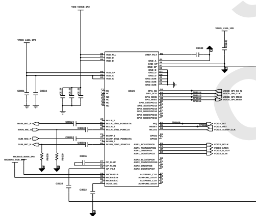
Voicewakeup IC
