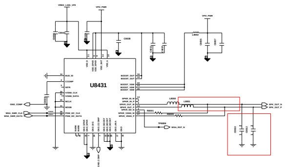
SPK IV SENSING BOOST AMP
